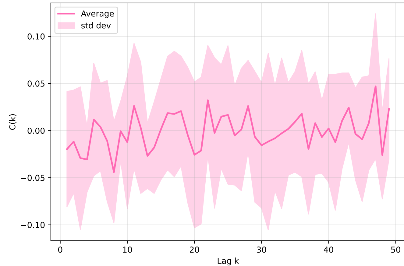
HOMO - Average autocorrelation for Experiment 0
