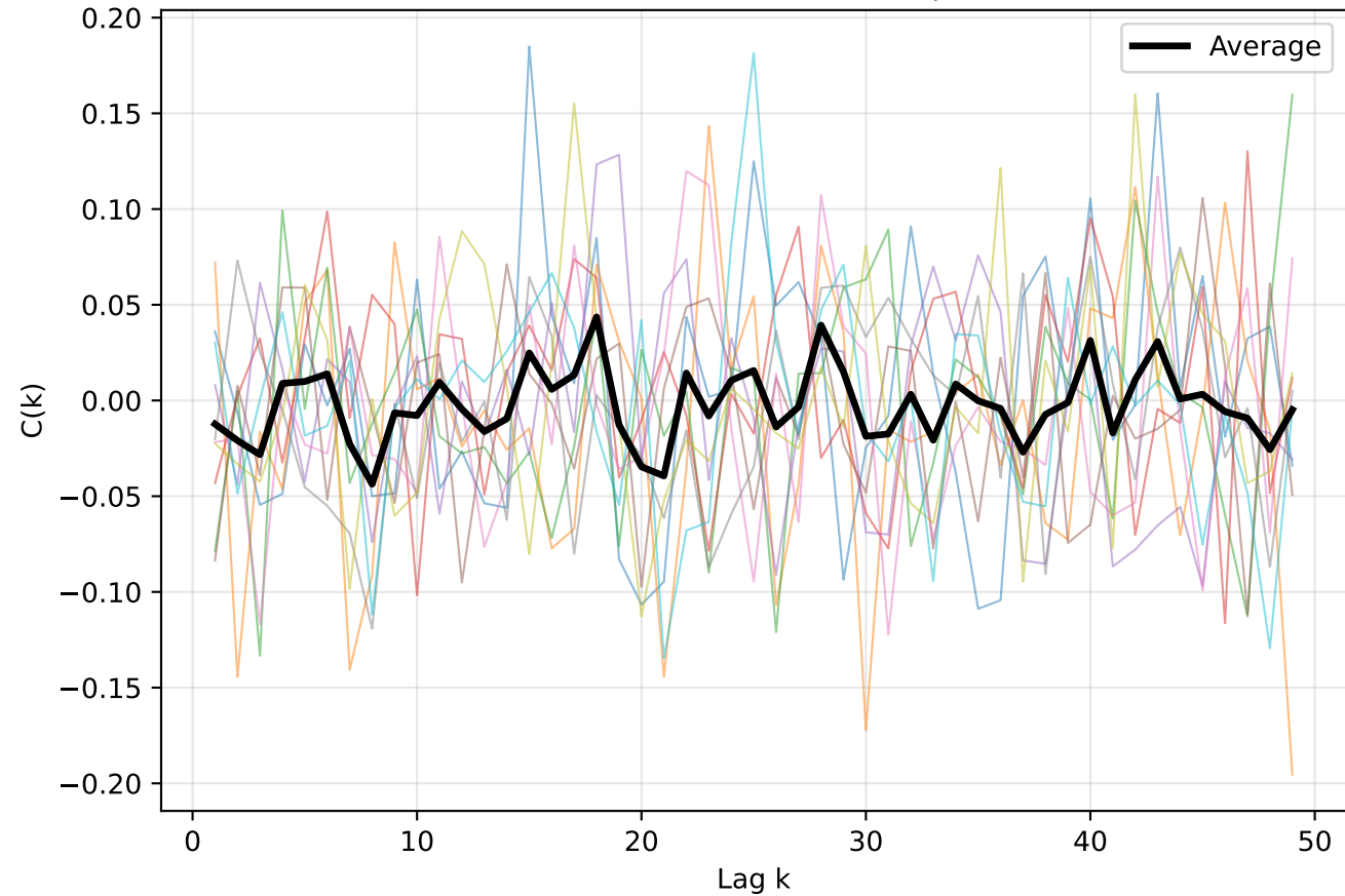
LUMO - All autocorrelation for Experiment 0
