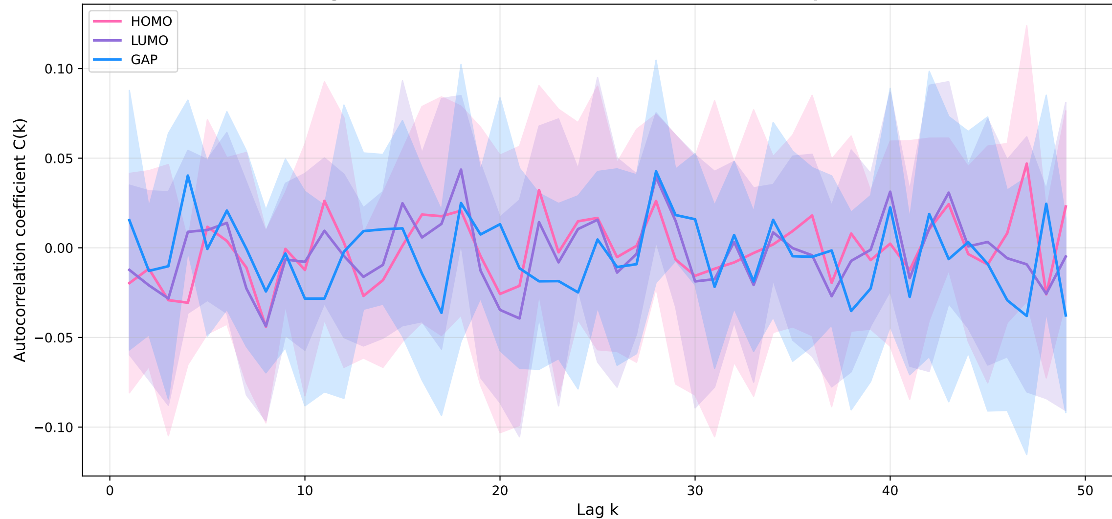
Average autocorrelations (HOMO, LUMO, GAP) for Experiment 0
