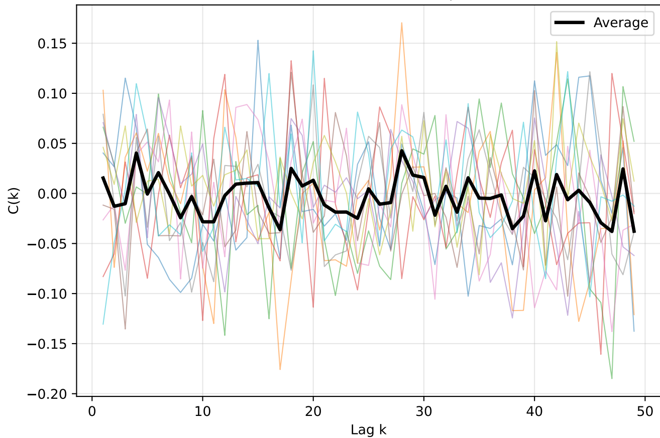
GAP - All autocorrelation for Experiment 0
