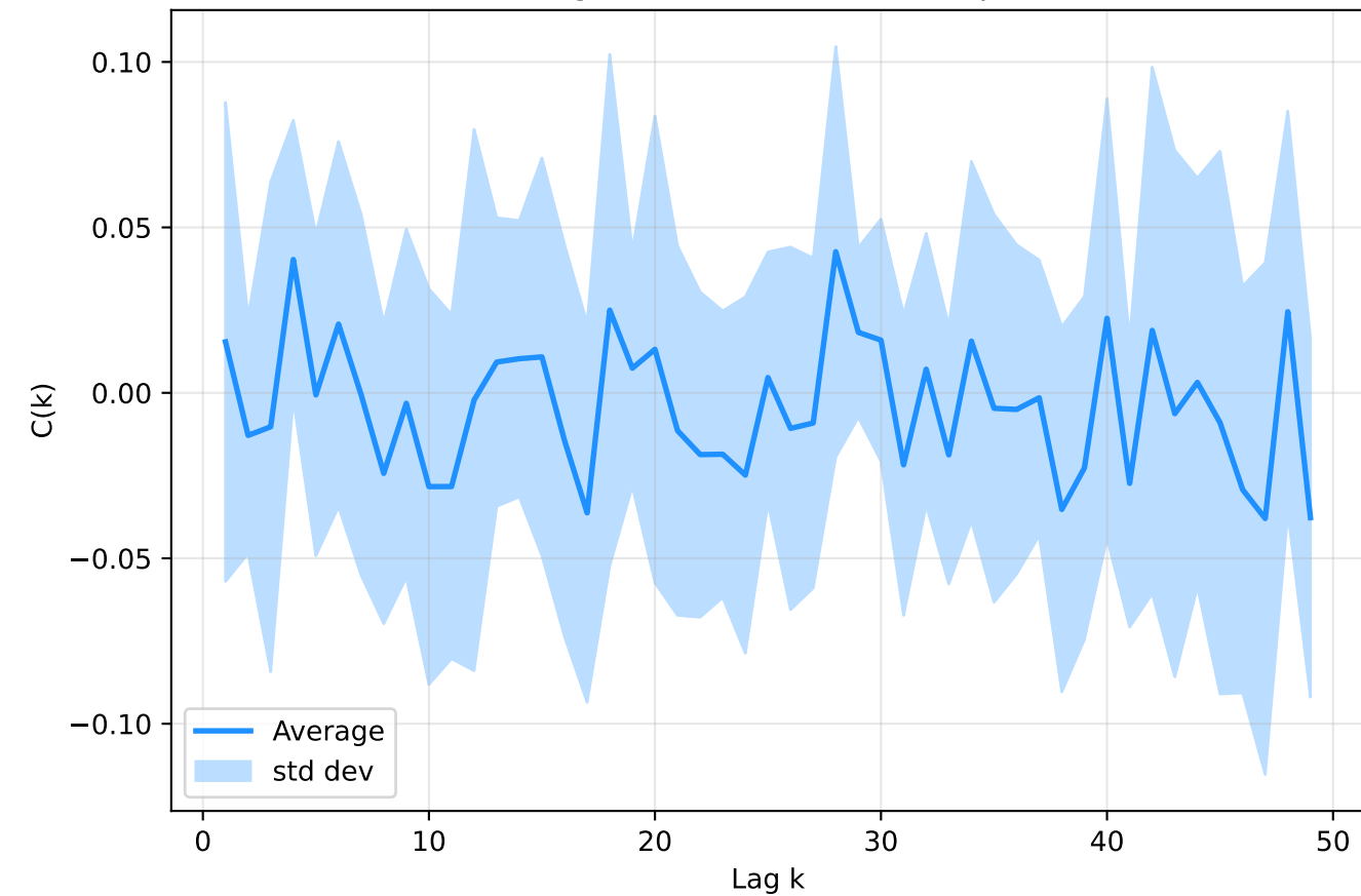
GAP - Average autocorrelation for Experiment 0
