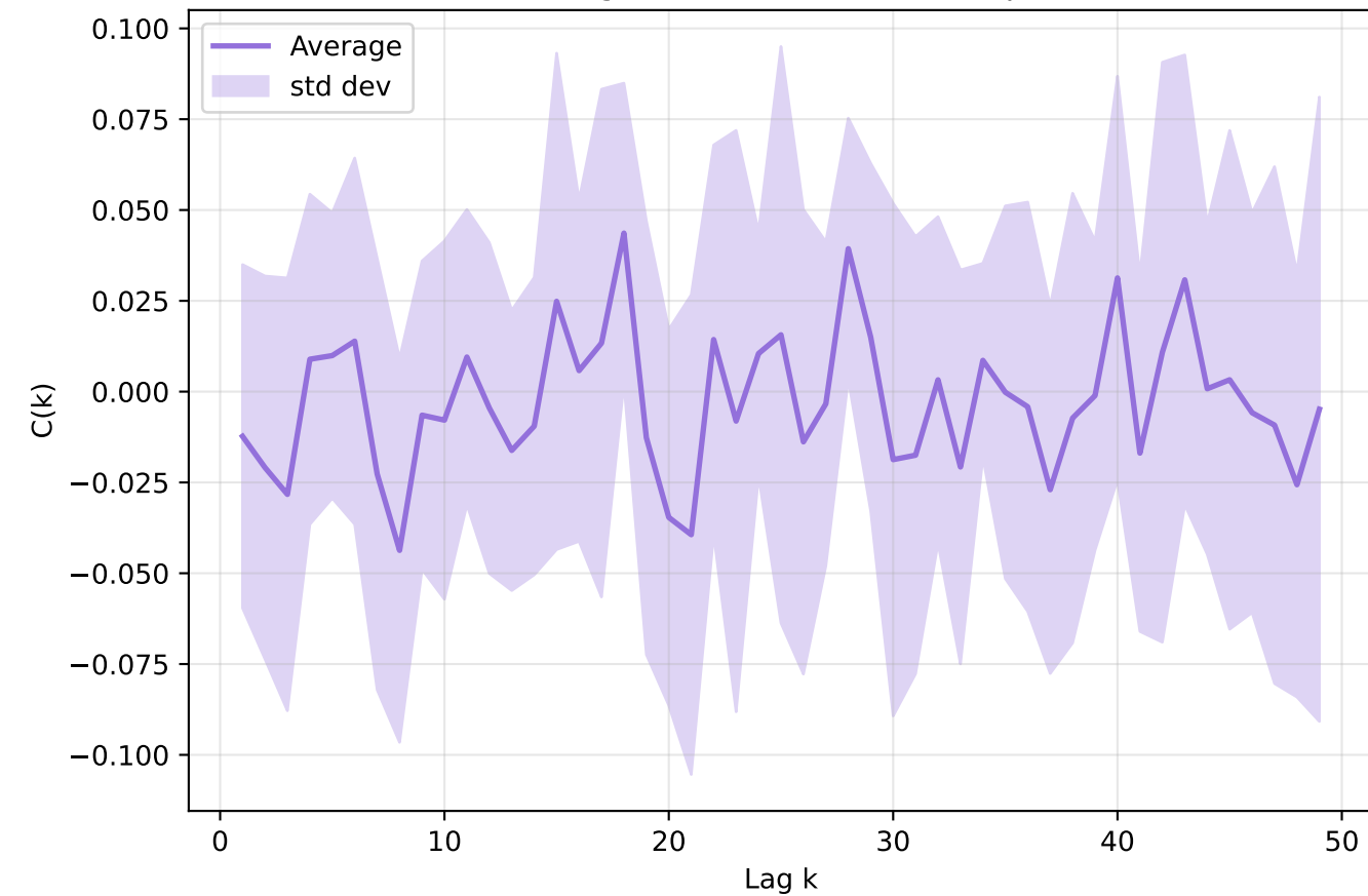
LUMO - Average autocorrelation for Experiment 0
