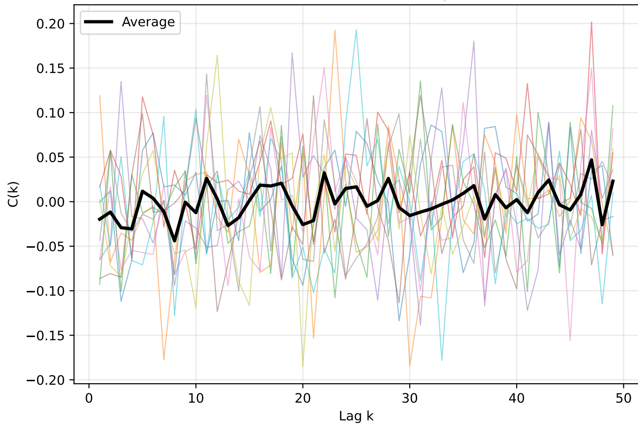
HOMO - All autocorrelation for Experiment 0
